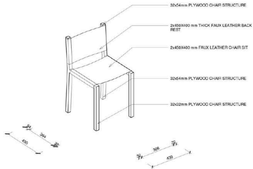
CHAIR ISOMETRIC SCALE 1:20
