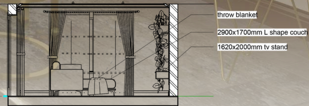
Livingroom elevation Scale 1:50
