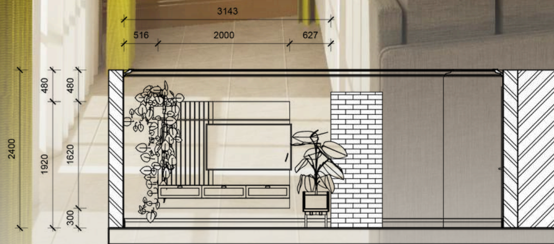
Livingroom Section Scale 1:50
