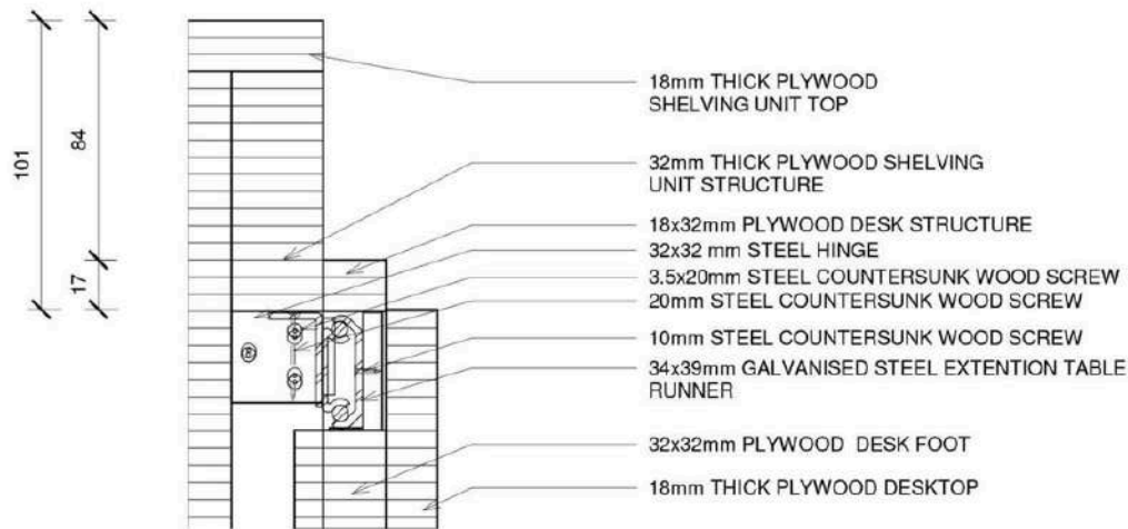
DETAIL 2 Scale 1:2
