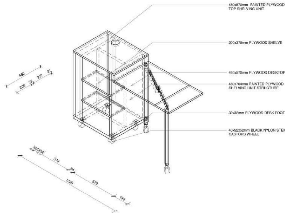
DESK ISOMETRIC SCALE 1:20
